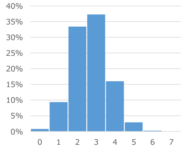
Aromatic Ring
