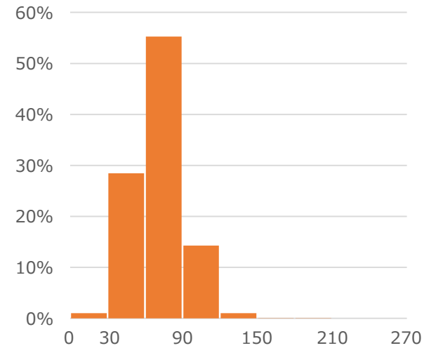
TPSA
