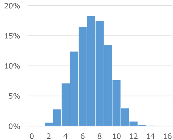
Rotable Bond
