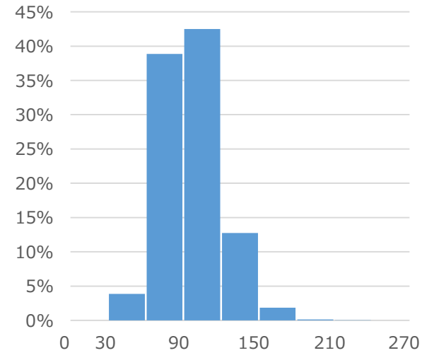
TPSA
