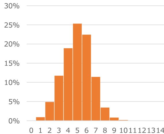
Rotable Bond
