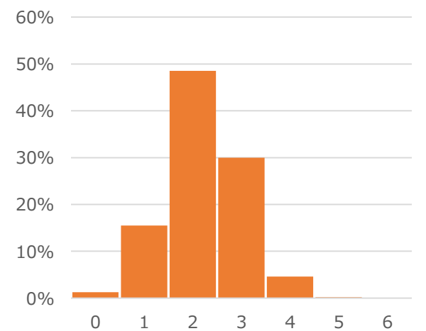
Aromatic Ring
