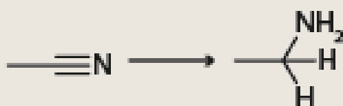
CN Bonds
