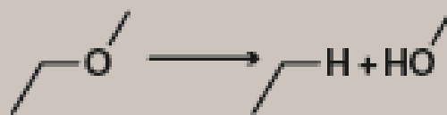
Hydrogenolysis
