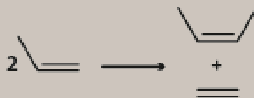
Metathesis
