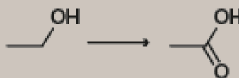
Dehydrogenations / Oxidations
