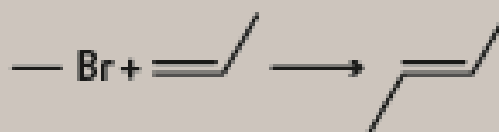
CC Coupling
